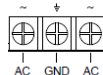
SCREW TERMINALS
